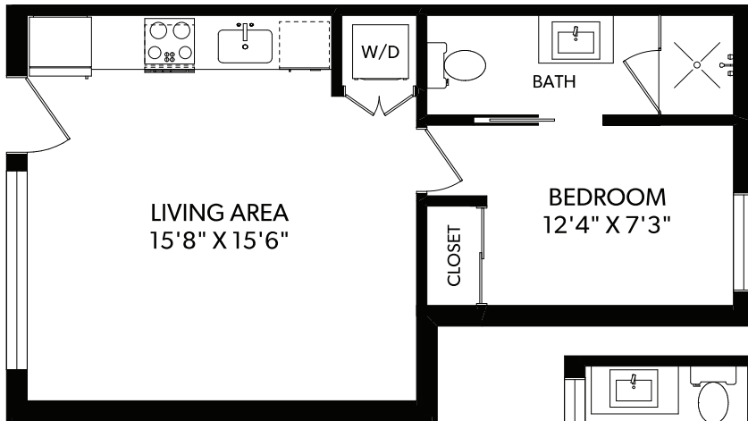
MAIN FLOOR (1A)
